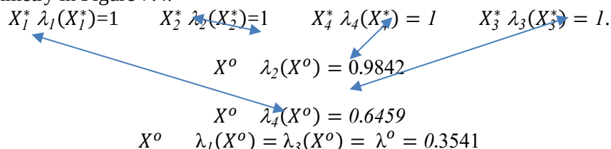
Figure 7.4. Geometric interpretation of symmetry in modeling of technical system with normalized criteria: \lambda_1(X), \dots, \lambda_4(X) .
