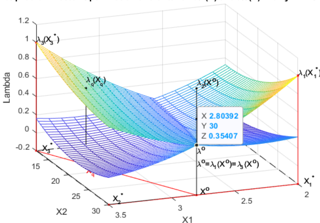
\lambda -problem Vector Optimization two criterion \lambda_1(X) and \lambda_3(X) . Машунин Ю.К.
