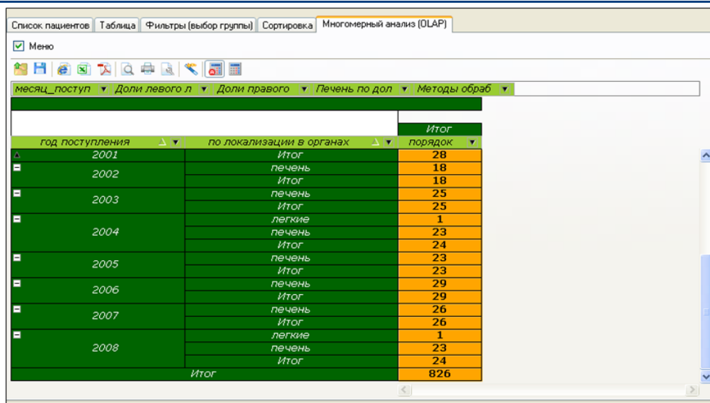
Figure 5. OLAP Multidimensional Analysis Window
